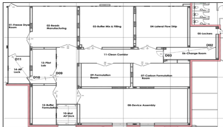
Figure 21 – Door Interlock Schedule Drawing GF (plan view)
