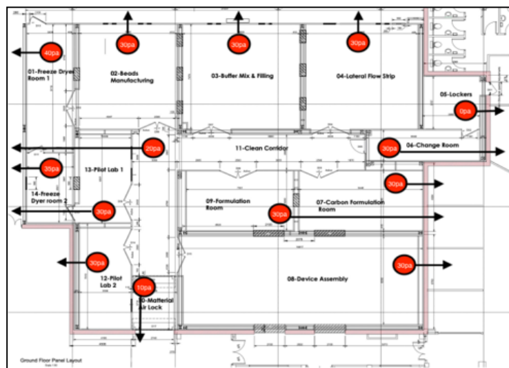
Figure 5 – Pressure Measurement Locations GF (plan view)
