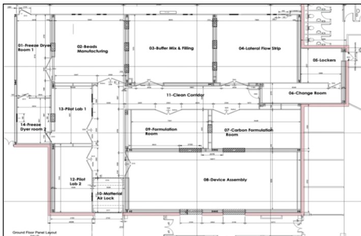
Figure 1 - Facility Layout Drawing Ground Floor (plan view)
