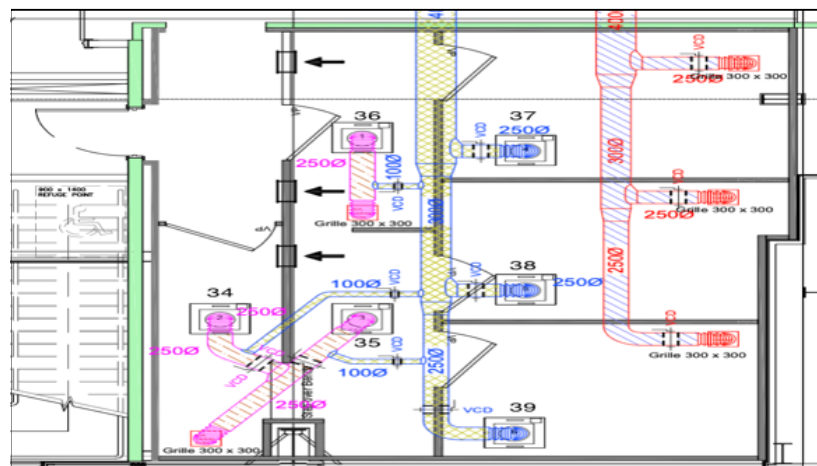
Figure 19 – Humidity Monitoring positions at bench height GF (plan view)
